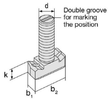
HBC-40/22-N, HBC-50/30-N
