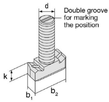
HBC-40/22-N, HBC-50/30-N
